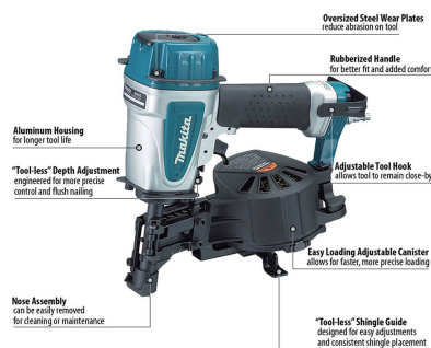
Makita AN453 Feature Shot (callouts)
