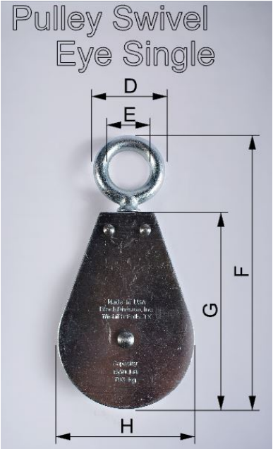
pulley swivel eye single
